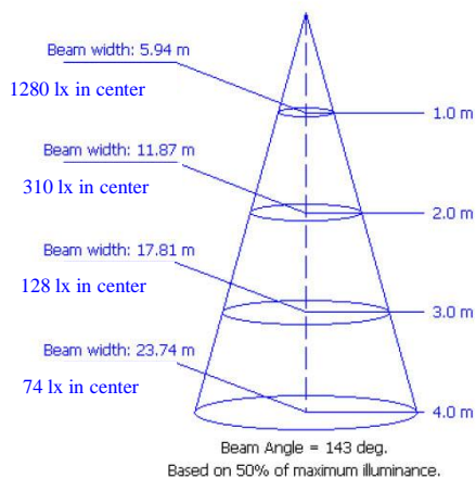
Illuminance Cone Diagram
